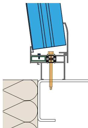
Detail Z
